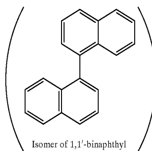
1,1'-binaphthyl
