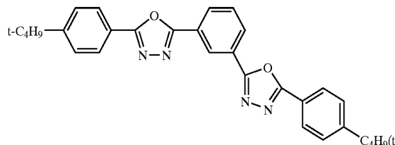
Zn(BOX) 2 Emission Material
